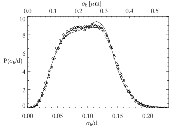
FIGURE 6. The distribution function P(\sigma_b/d) for tetrahedral “irregularity” for three ages: \triangle : t_w = 0 , \times : t_w = 100\tau_{\text{diff}} , and \circ : t_w = 300\tau_{\text{diff}} . The solid line is a reference curve computed by considering random bonds based on g(r) , without the constraint that such bonds form a tetrahedron.
