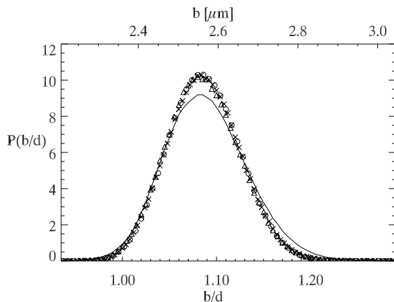
FIGURE 5. The distribution function P(b/d) for tetrahedral bond lengths (“looseness”) for three ages. \triangle : t_w = 0 , \times : t_w = 100\tau_{\text{diff}} , and \circ : t_w = 300\tau_{\text{diff}} . The solid line is a reference curve computed by considering random bonds based on g(r) , without the constraint that such bonds form a tetrahedron.
