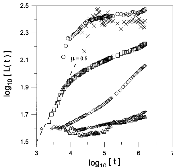
FIG. 2. Average linear crystal dimension L(t) [Eq. (3)] versus dimensionless time. Symbols are as indicated in Fig. 1.
