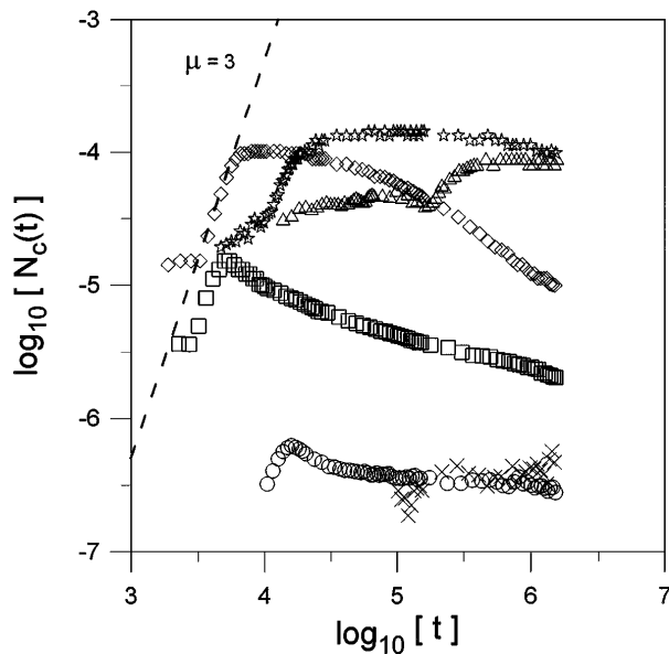
FIG. 3. Number density of crystals N_c(t) [Eq. (4)] versus dimensionless time. Symbols are as indicated in Fig. 1.
