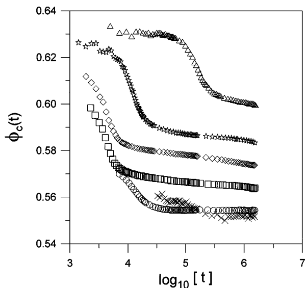
FIG. 5. Volume fraction of the crystal phase, calculated from the Bragg peak positions [Eq. (5)], versus dimensionless time. Symbols are as indicated in Fig. 1.
