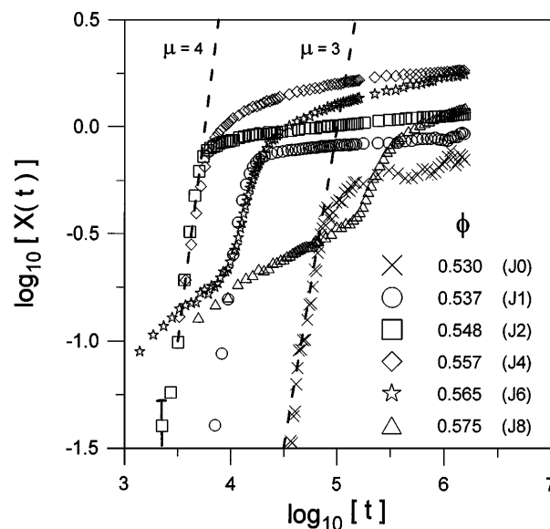
FIG. 1. Degree of crystallinity X(t) [Eq. (2)] versus dimensionless time t expressed in units of \tau_b = a^2/D_0 , where D_0 is the free particle diffusion coefficient. Effective hard sphere volume fractions \phi and our designations are indicated. Power laws t^\mu are shown by dashed lines with indicated exponents \mu . Estimates of uncertainties incurred in the measurements and background subtraction are indicated for X(t) \leq 0.1 . These are negligible for X(t) \geq 0.1 .
