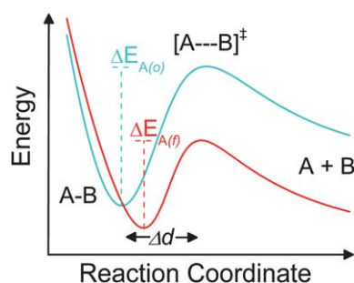
Fig. 2 Representation of the potential energy surface of a reaction in the absence of a coupled force (blue) and in the presence of a coupled force (red). The force leads to a net reduction in activation energy of \Delta(\Delta E_{\text{act}}) = \Delta E_{A(o)} - \Delta E_{A(f)} . Note that eqn (1) in the text assumes that the distance \Delta d from reactant to transition state does not change as a function of force, but that perturbations are possible.
