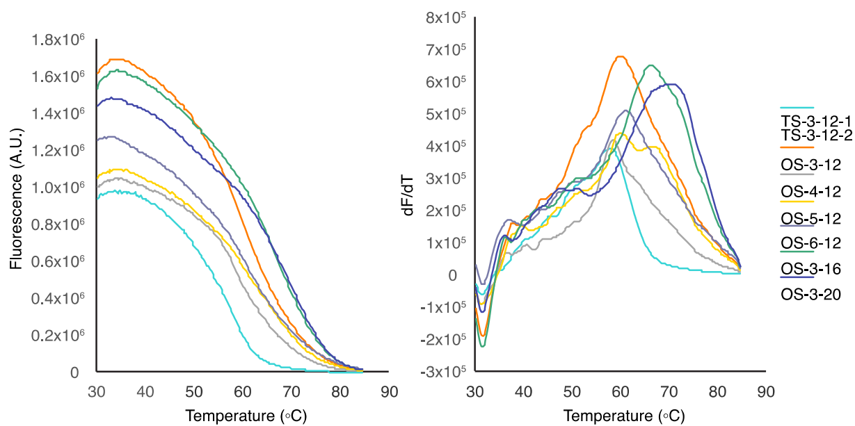
Figure S1. Melting temperatures of OS strands and TS strands. Left: fluorescence vs. temperature. Right: derivatives of fluorescence vs. temperature.
