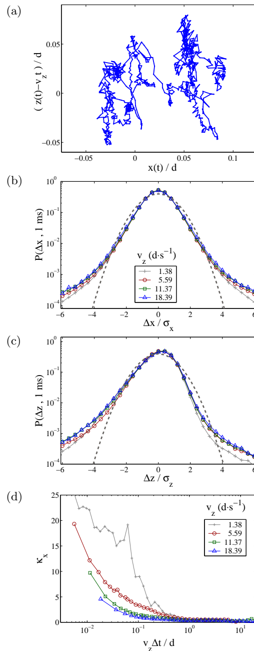
FIG. 2: (a) A typical particle trajectory sampled at 1 ms intervals in a frame moving with the average flow speed, v_z . (b)–(c) Normalized PDFs for the 1 ms particle displacements, \Delta x and \Delta z , for various flow speeds, v_z , compared to a standard Gaussian distribution (dotted line); standard deviations, \sigma_x and \sigma_z , are of order 10^{-3}d . (d) The kurtosis of \Delta x versus the mean distance fallen, v_z \Delta t .
