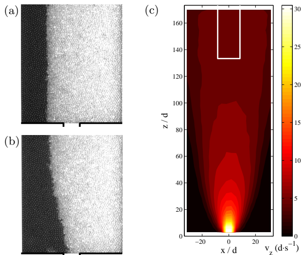
FIG. 1: An initially flat, off-center interface between two regions of differently colored beads (a) stretches and roughens after draining half of the silo (b), but little mixing is observed. (c) Contour plot of the average downward velocity field, v_z , with an orifice width, W = 16 \text{ mm} = 5.3 d , where d is the particle diameter. The white box indicates a region of nearly uniform flow where all subsequent measurements are made.
