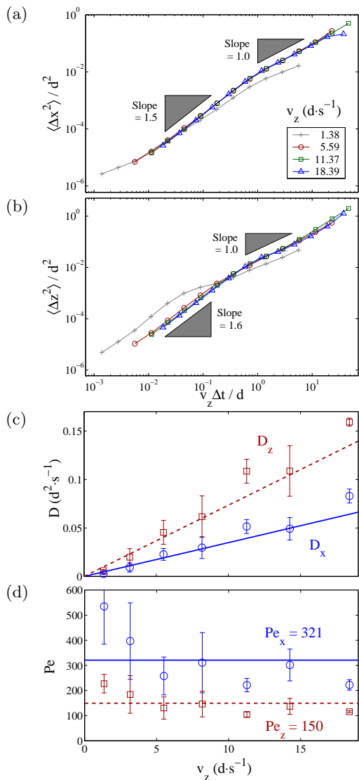
FIG. 3: (a)–(b) Mean squared horizontal ( \langle \Delta x^2 \rangle ) and vertical ( \langle \Delta z^2 \rangle ) displacements versus mean distance dropped, which collapse onto a single curve for different flow speeds, v_z , except for the smallest where the flow is intermittent. (c)–(d) Diffusion coefficients ( D ) and Péclet numbers ( Pe ) in the horizontal ( x ) and vertical ( z ) directions versus v_z .
