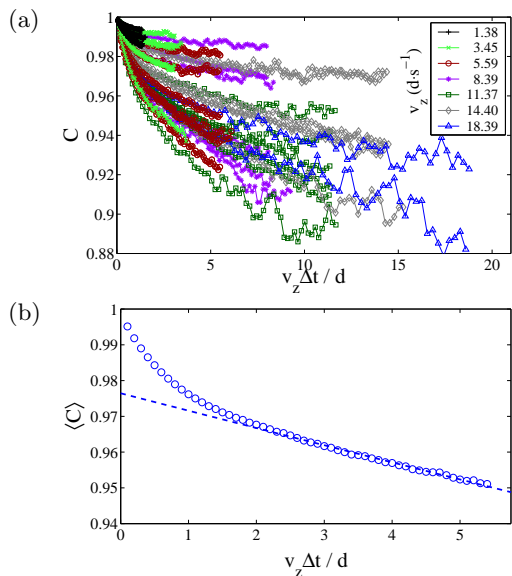
FIG. 4: (a) The topological cage correlation function, C(\Delta t) , versus the mean distance fallen, v_z \Delta t , and (b) the average over all experiments in the continuous-flow regime ( W \geq 16 mm), compared with an exponential fit in the diffusive regime (dotted line).
