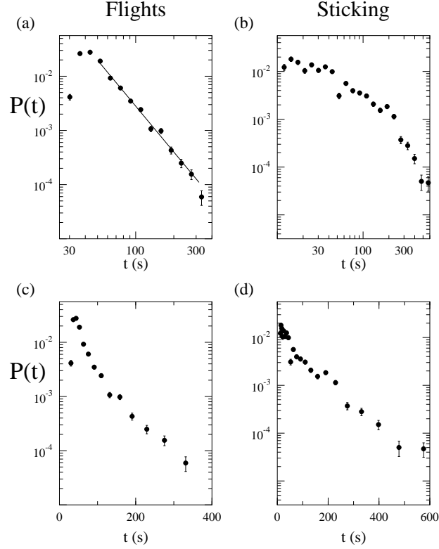
Fig. 12. Six-vortex flow: (a,c) flight and (b,d) sticking probability distribution functions, shown on (a,b) log-log axes and (c,d) log-linear axes. The error bars show the statistical uncertainty ( \sqrt{N} ). The flight PDF shows power law decay, P_F \sim t^{-\mu} ; the line drawn in (a) is a least squares fit to the decaying data yielding \mu = 2.5 \pm 0.2 . The sticking PDF does not show a clear power law decay nor an exponential decay. Note that these PDFs are slightly different from those shown in Refs. [9], [10] due to the improvement in binning technique (Sec. 3.2). (The uncorrected value of \mu is 2.8 \pm 0.2 ; see Sec. 3.2 for details of the correction.)
